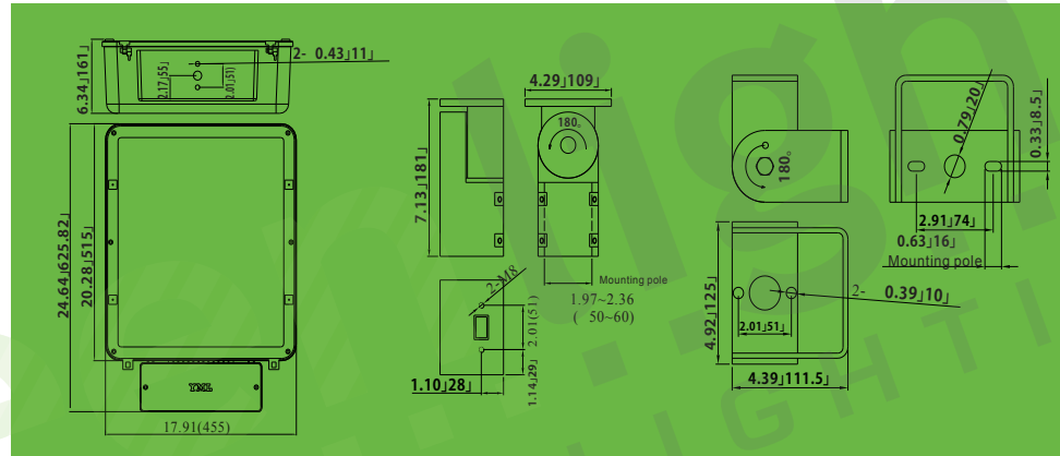
Fixture sizes (Unit: mm)
