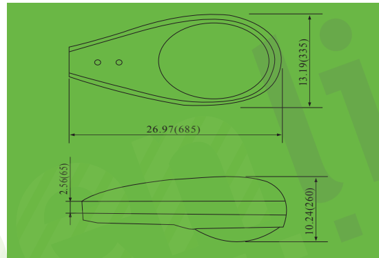
Fixture sizes (Unit: mm)
